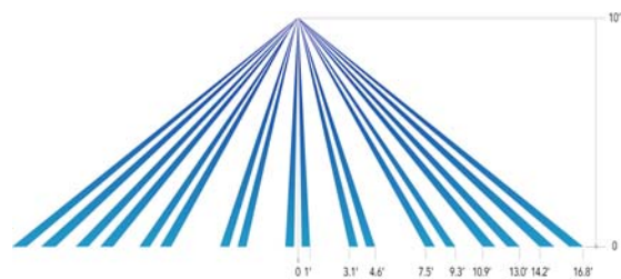
Protection Pattern Dimensions in ft. (m)
