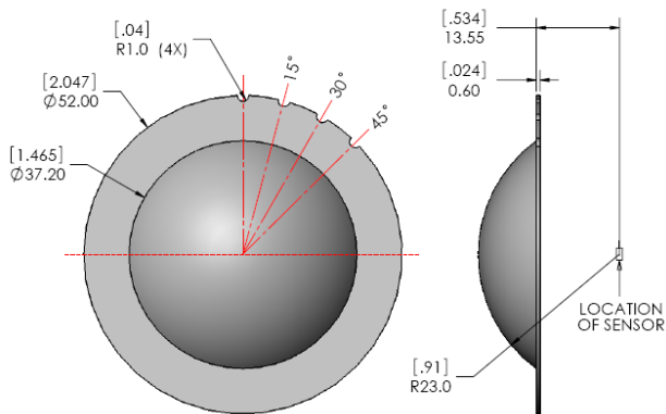
Dimension Schematic Ceiling Lens Array
