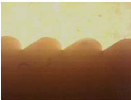
A cross section view of an injection molded Fresnel lens shows poor microstructure replication
